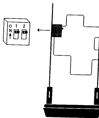
Control Chassis - Bottom View
