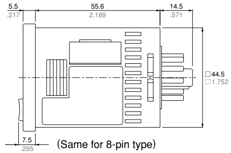
Pin type (embedded installation/ front panel installation)
