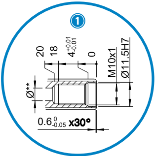
Connection details (thread core)
