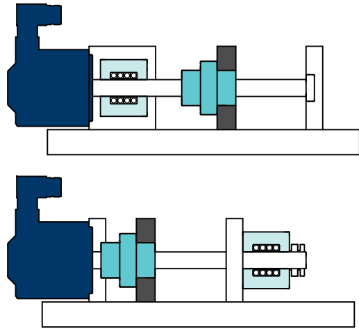
Bearing assembly "single / double"
