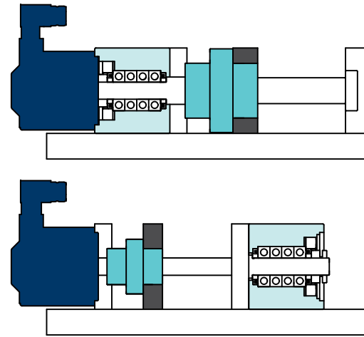
Flange bearing unit
