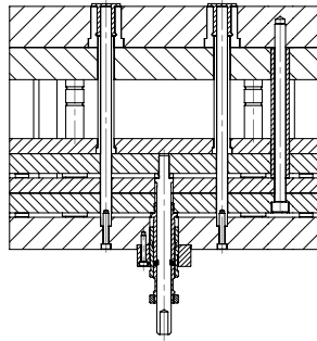
SECTION B-B EJECTOR PLATES BACK - MOLD OPEN
