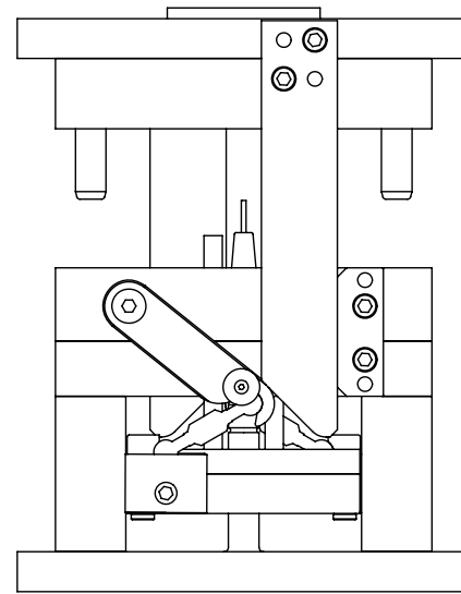
MOLD CLOSING
